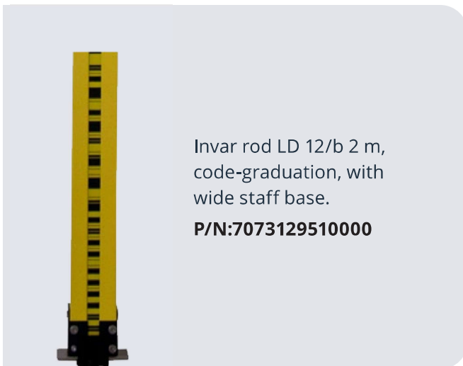
Leveling Staff LD 12/b
