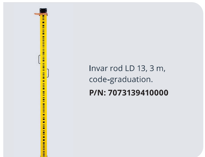
Leveling Staff LD 13
